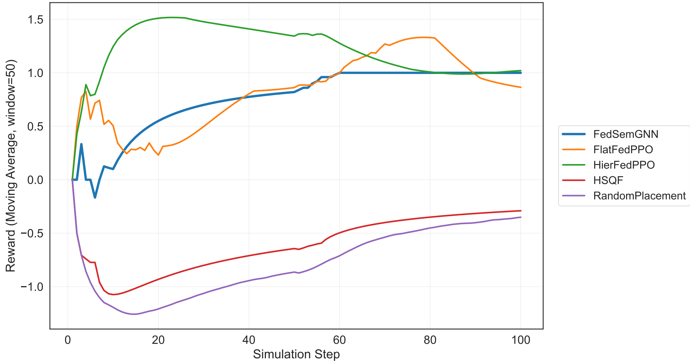
Temporal Reward Progression Across All Algorithms [TEMPORAL ANALYSIS: Learning Evolution, Moving Window=50 steps]
